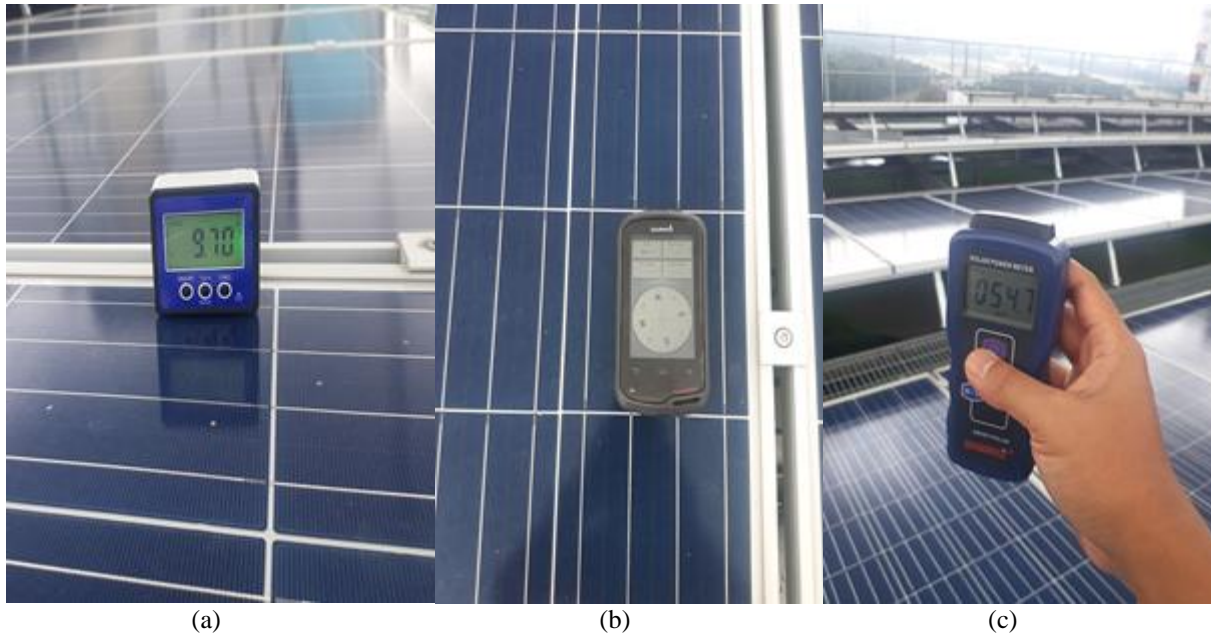
Figure 8. Data collection conditions for (a) module slope angle, (b) module orientation, and (c) radiation intensity.
