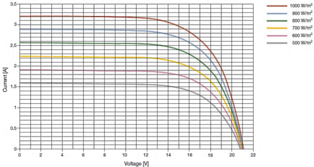
Figure 1. Graph of function I and V towards solar radiation.
