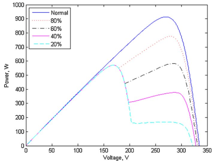
Figure 5. Effects of shading on power solar modules.
