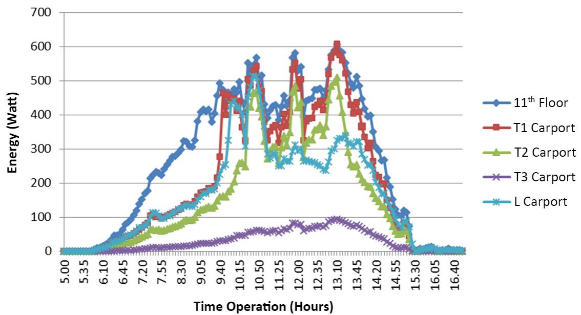
Figure 12. Graph of PLTS daily energy on December 22, 2019.
