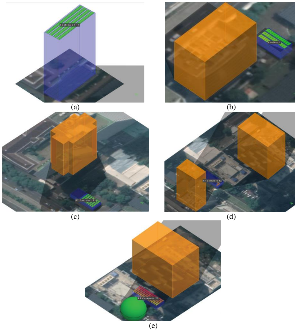
Figure 11. Display of 3D shading of the solar power plants of Setjen KESDM.
