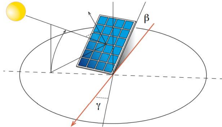
Figure 3. Optimal position of solar module placement.
