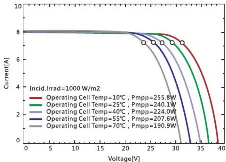
Figure 2. Graph of function I and V towards temperature.
