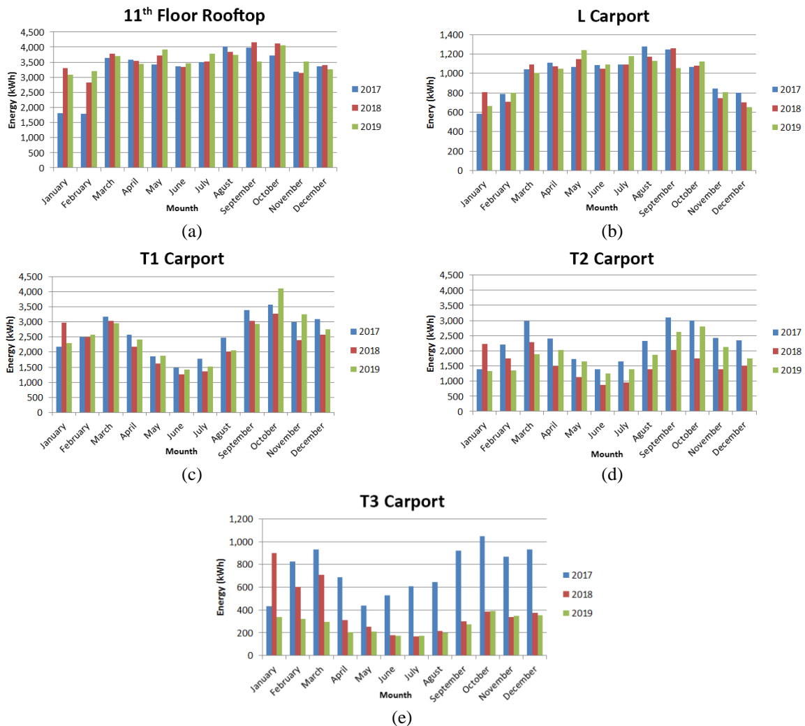
Figure 10. Graph of energy production of the solar power plants on (a) 11 th floor rooftop, (b) L carport, (c) T1 carport, (d) T2 carport, and (e) T3 carport.
