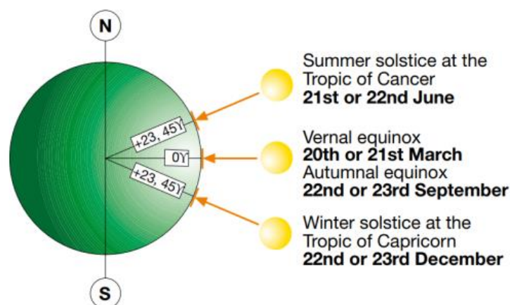
Figure 4. Changes in solar declination angle in one year.
