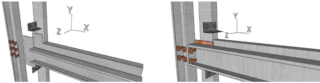
Image 1. Illustration of test object, (a) screw connection, (b) screw-gusset plate connection, (c) angle cleats-screw connection, (d) gusset plate-plate joint
