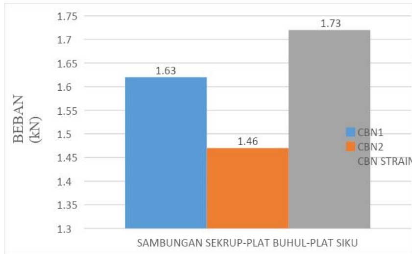
Figure 6. Graph of the connection strength of the screw-gusset plate-angle cleats
