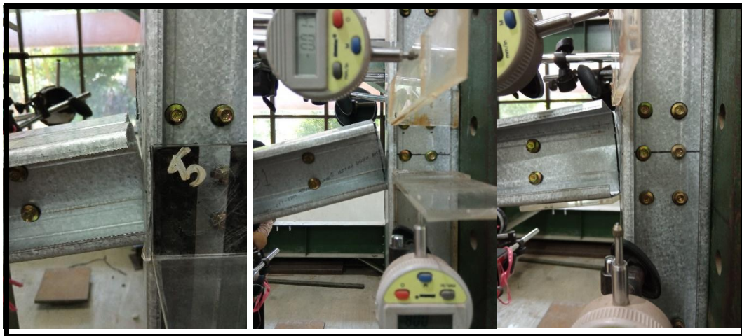
Figure 4.10. Failur at the Screw Joint
