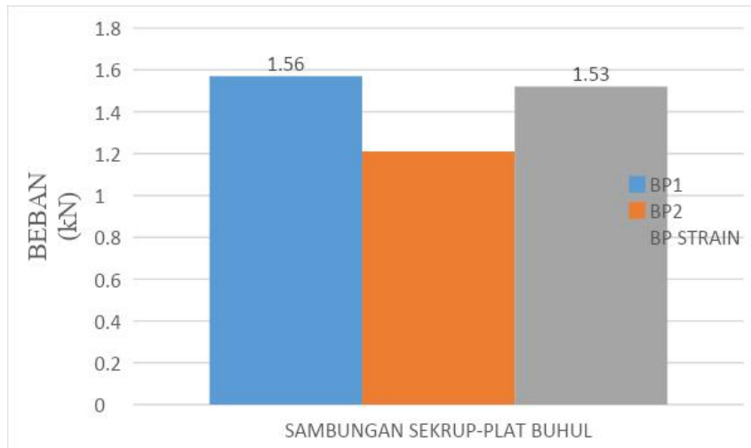
Figure 4. Strength Graph of the Bolt-Gusset Plate Joint
