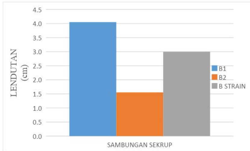
Figure 7. Screw Connection Deflection Graph
