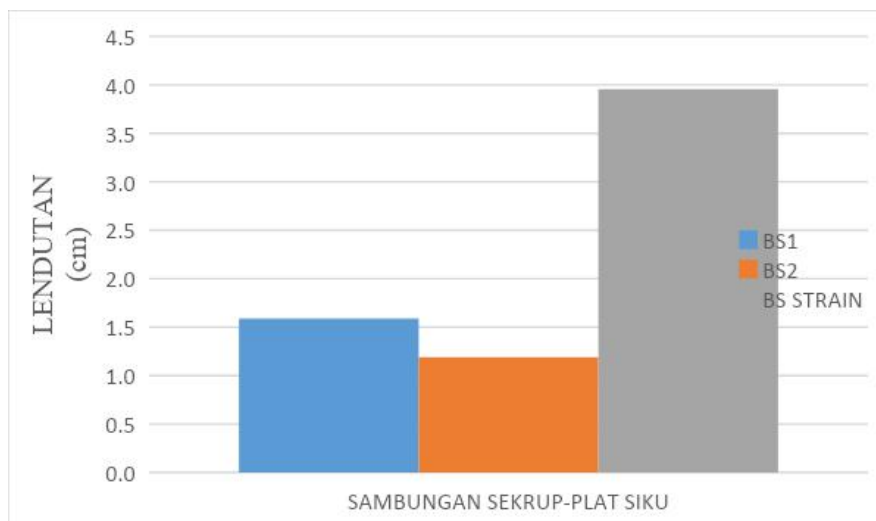
Figure 9. Deflection Graph of Angle cleats-Screw Connection
