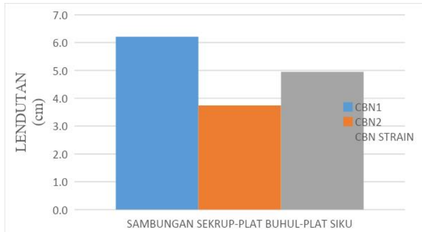
Figure 4.10. Deflection Graph of the Screw-Tush Plate-Angle cleats
