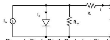
Figure 1. Single-Diode Equivalent Circuit
