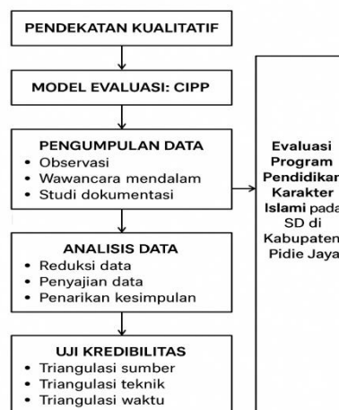
Gambar 1. Flowchart penelitian
