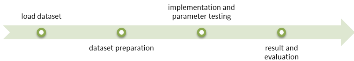
Fig. 1. Research methodology
